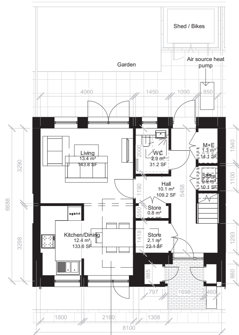
Plot No. C-017 3B5P M4(2) H-3B 46 m²
