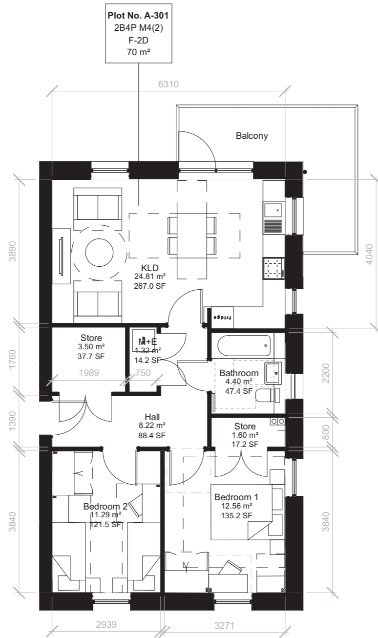
Flat Type F-2D
