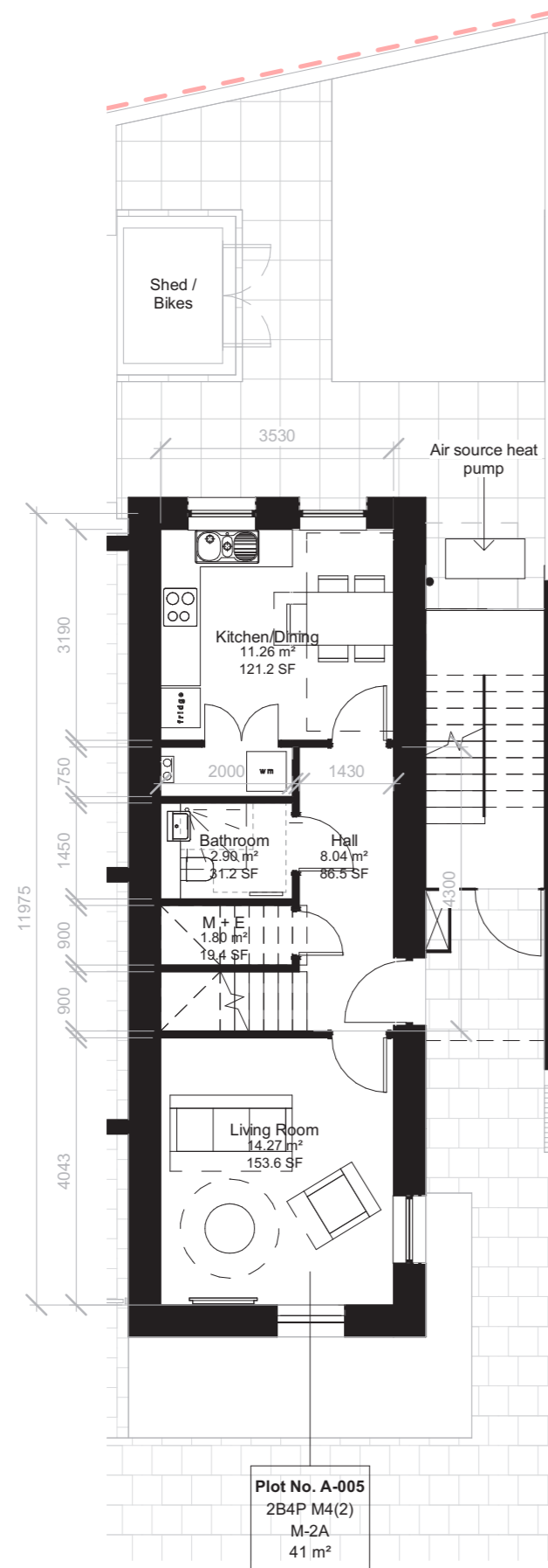
Entry Level (Ground Floor)
