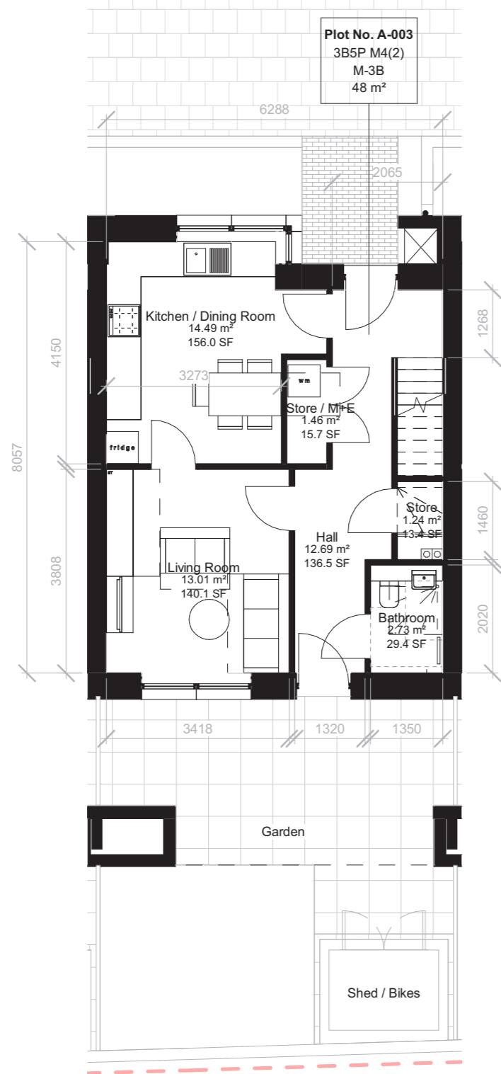
Entry Level (Ground Floor)
