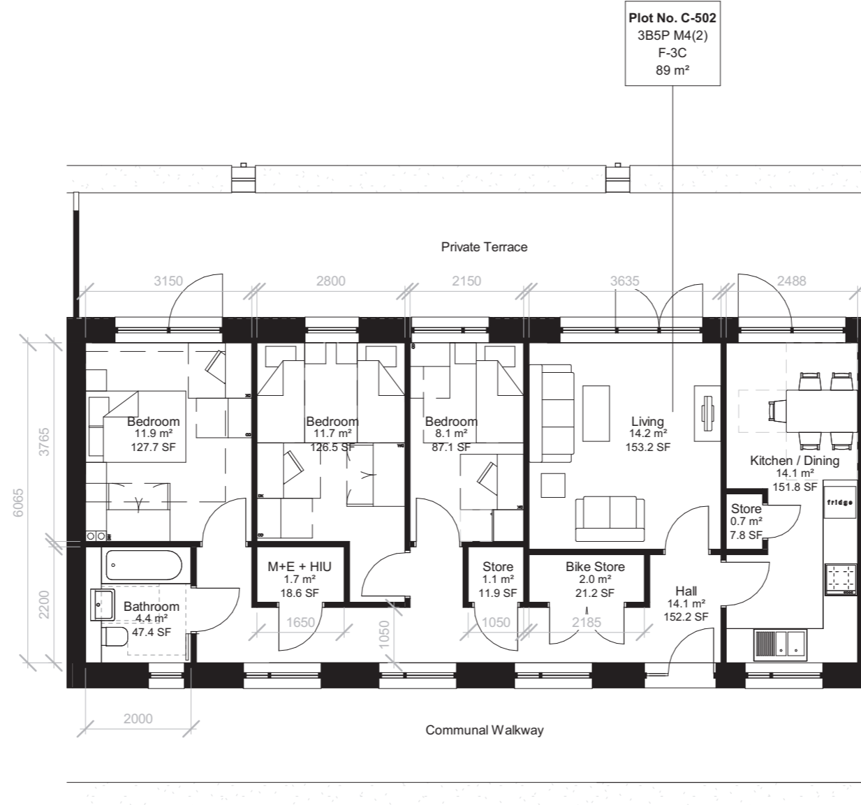
Flat Type F-3C
