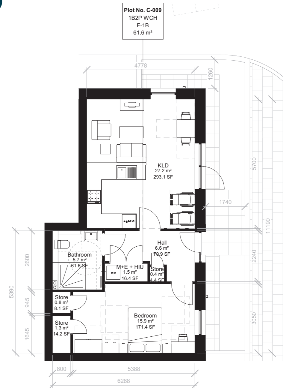
Flat Type F-1B (wch)
