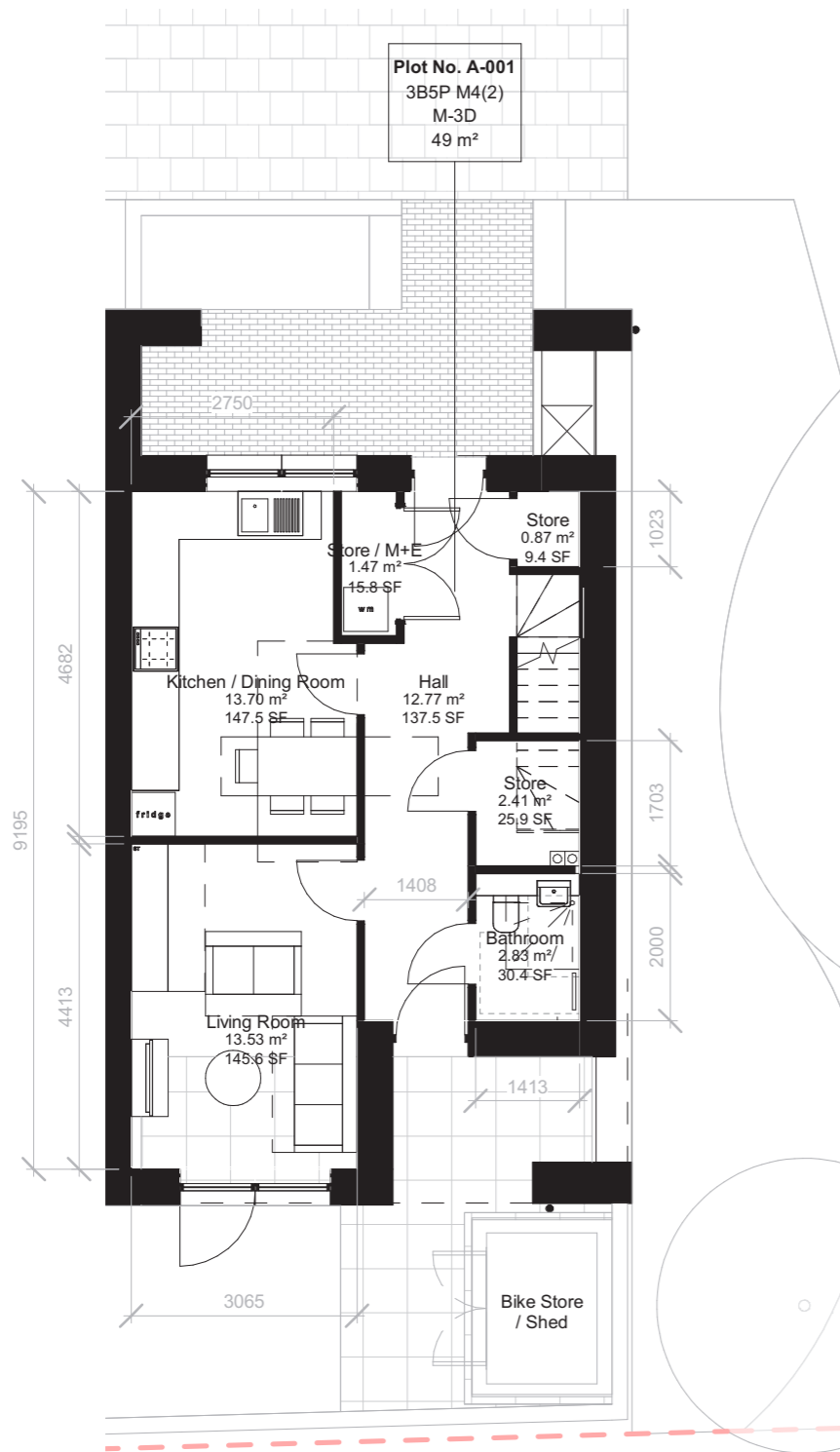
Entry Level (Ground Floor)
